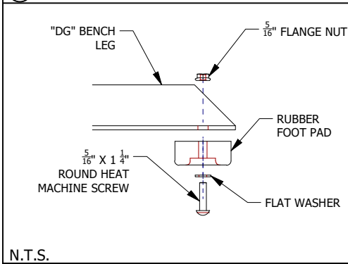
① RUBBER FOOT PAD ASSEMBLY
