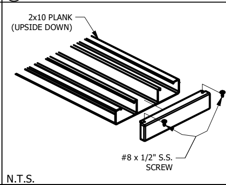
⑥ CROSS BRACE CENTER CONNECT.
