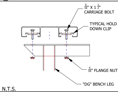
⑤ TYP. BRACING ATTCHMENT
